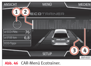
Abb. 46 CAR-Menü Ecotrainer.
