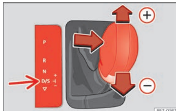
Abb. 99 Hebel in Tiptronic-Stellung.
